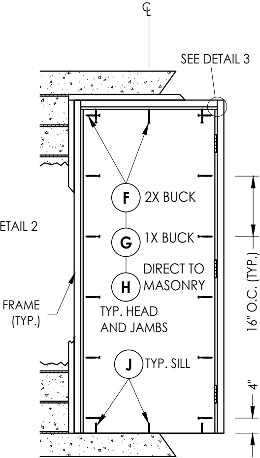
FRAME ANCHORING Max. D.P. <= 70 PSF
