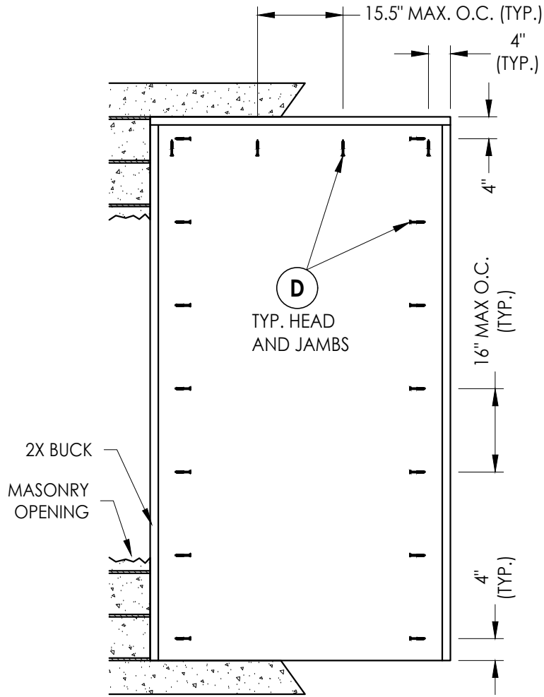
BUCK ANCHORING
